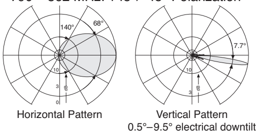
790 – 862 MHz: +45°/–45° Polarization
